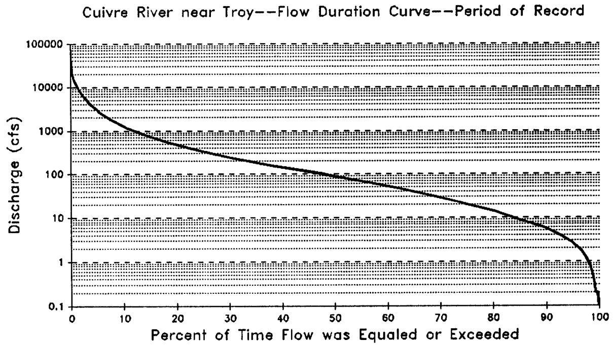
Figure 7. Flow duration curve for the Cuivre River near Troy, gage station #05514500, 1923 to 1972 and 1979 to 1985.
