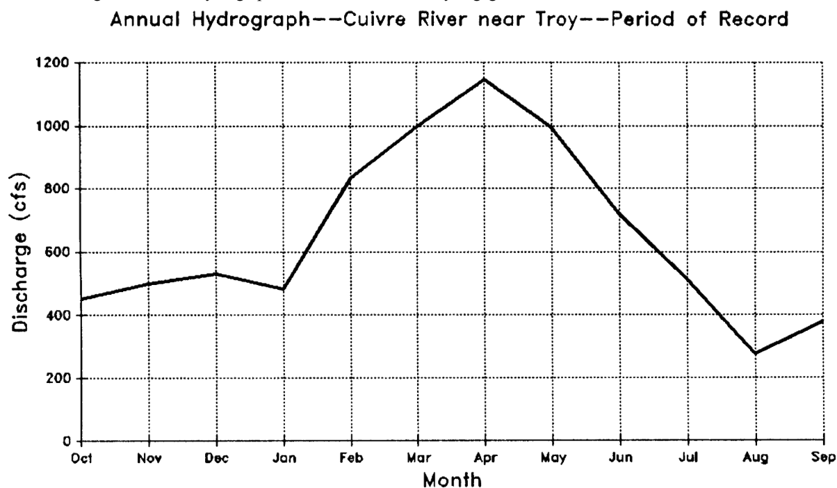
Figure 6. Annual hydrograph of Cuivre River near Troy at gage #05514500, 1922 to 1972 and 1979 to 1990.
